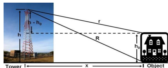
Figure 2: Single tower with an object.
