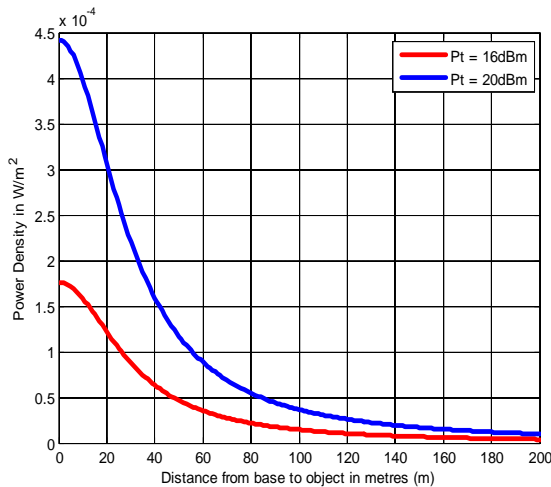
Figure 2: Power density versus distance of a point for P_t = 16dBm , 20dBm and a gain G_t = 17dB
