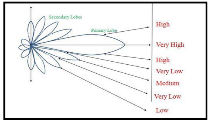
Figure 1: Radiation Pattern of Cell Tower Antennas
